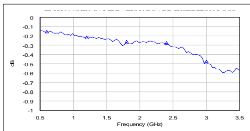
Insertion Loss
