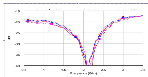
Return Loss
