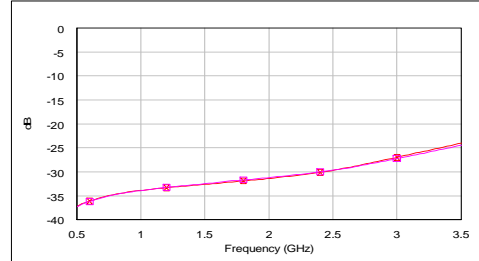
RF1 to RF2 Isolation
