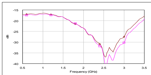
Return Loss
