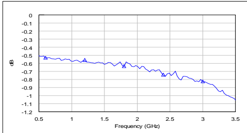
Insertion Loss
