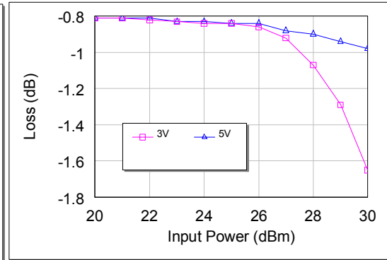
Insertion Loss vs. Power
