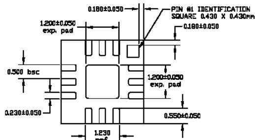
Btm View
