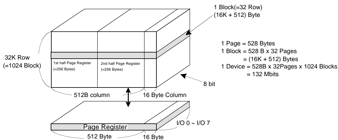
Figure 2. ARRAY ORGANIZATION
