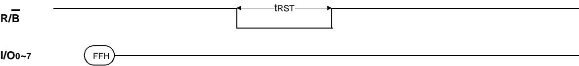
Figure 10. RESET Operation
