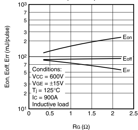
Rg-Esw (TYPICAL)
