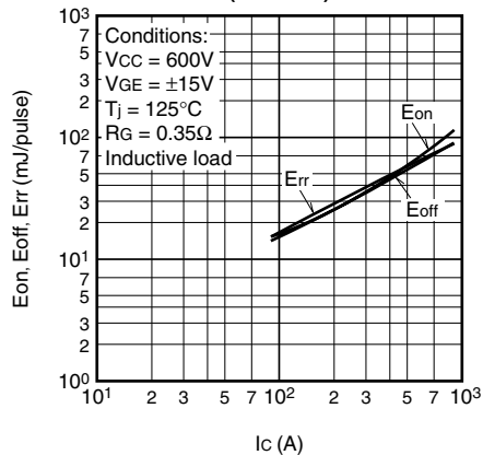
Ic-Esw (TYPICAL)
