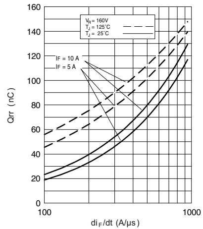
Fig. 8 - Typical Stored Charge vs. di_F/dt
