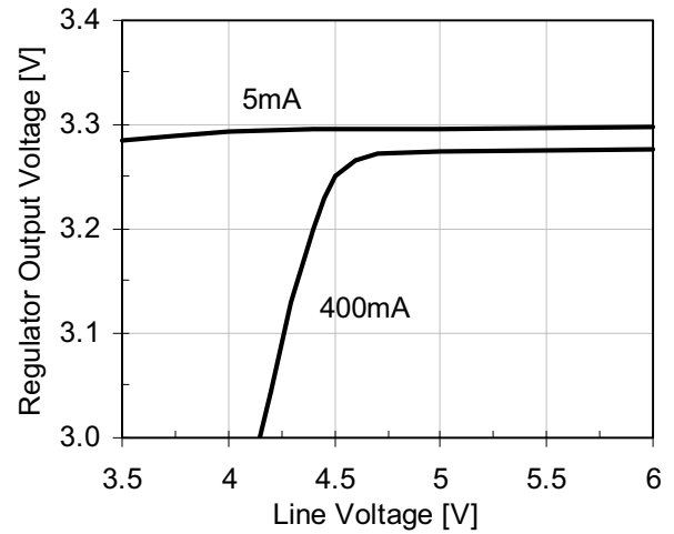
Line Regulation
