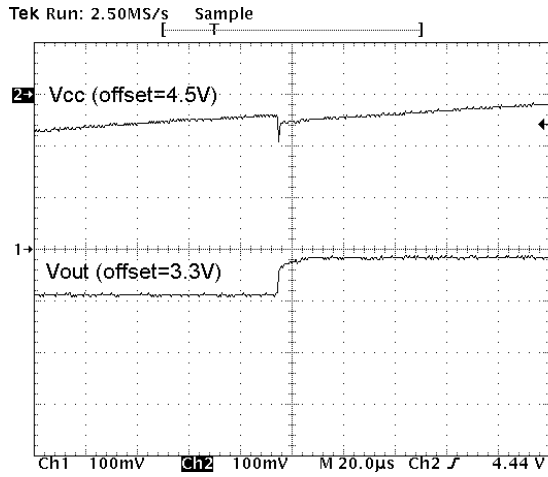
V_{CC} power up ( V_{AUX} = 3.3V , Load = 300mA)
