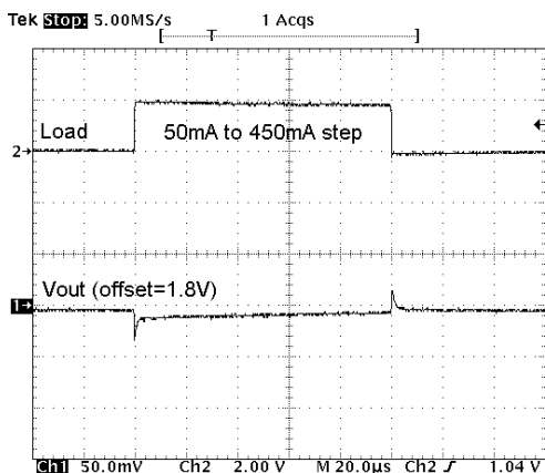
Load Transient Response (50mA to 500mA)
