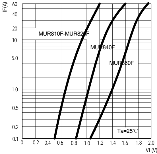
图3: 正向电压曲线 FIG3: Instantaneous Forward Voltage
