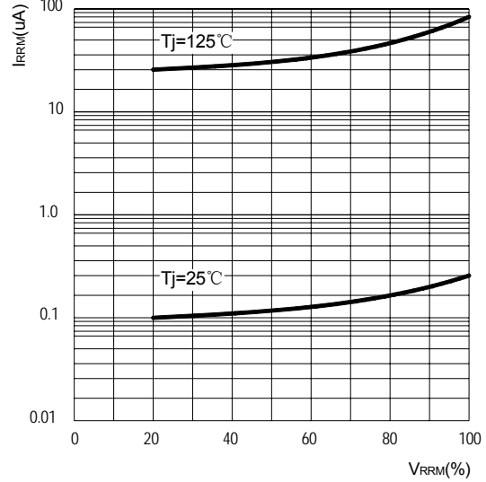
图4: 反向电流曲线 FIG4: Typical Reverse Characteristics
