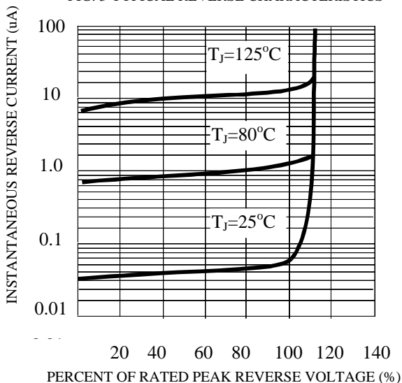
FIG. 3-TYPICAL REVERSE CHARACTERISTICS
