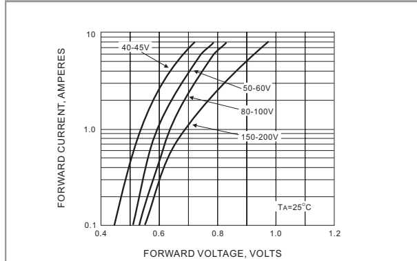
Fig.2- TYPICAL INSTANTANEOUS FORWARD CHARACTERISTIC
