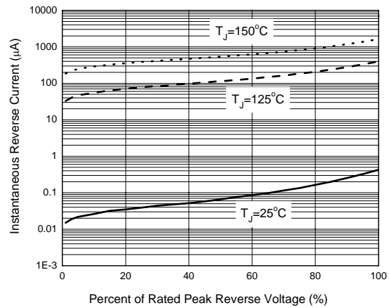
Figure 5. Typical Reverse Current Per Diode
