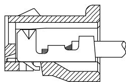
TERMINAL ASSEMBLY DRAWING
