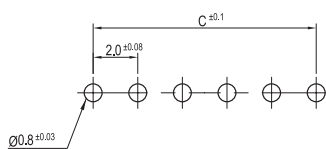
PCB LAYOUT
