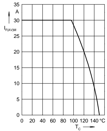
Fig. 5 Max. forward current versus case temperature
