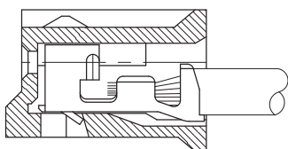
TERMINAL ASSEMBLY
