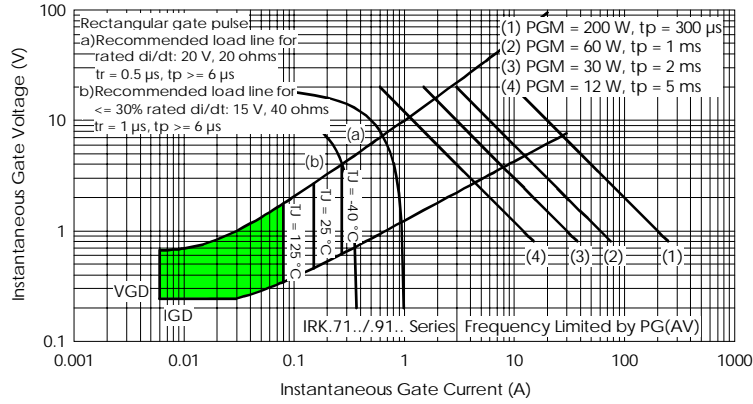
Fig. 24 - Gate Characteristics
