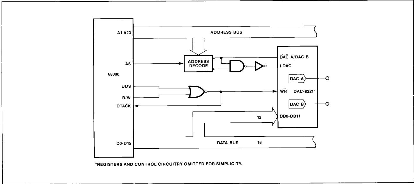
FIGURE 10: DAC-8221 To 68000 Interface
