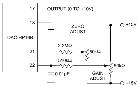
Figure 3. Unipolar Operations
