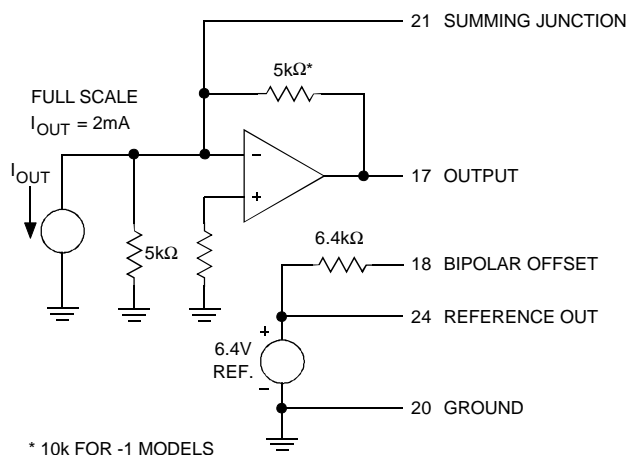
Figure 5. Output Circuit
