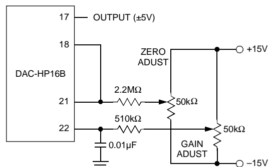
Figure 4. Bipolar Operations
