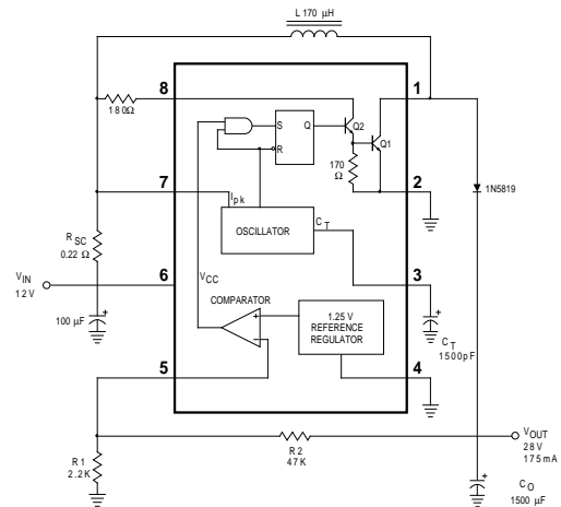
Step-Up Converter
