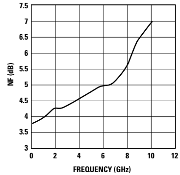
Figure 3. NF vs. Frequency at I_d = 50 mA.
