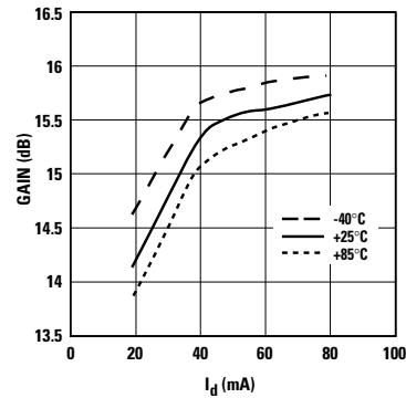
Figure 6. Gain vs. I_d and Temperature at 2 GHz.
