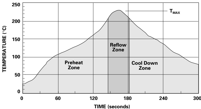
Figure 12. Surface Mount Assembly Profile.
