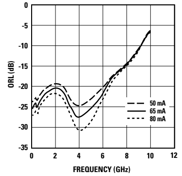
Figure 15. Output Return Loss vs. I_d and Frequency.
