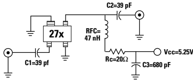
Figure 8. Schematic of 900 MHz Circuit.
