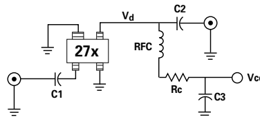
Figure 1. Schematic Diagram with Bias Connections.
