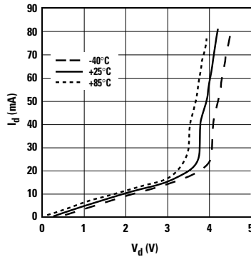
Figure 5. I_d vs. V_d and Temperature.
