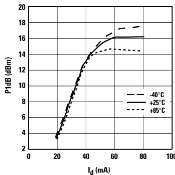
Figure 8. P1dB vs. I_d and Temperature at 2 GHz.
