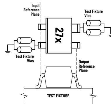
Figure 11. Phase Reference Planes.
