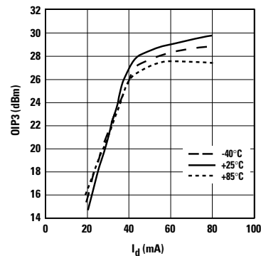
Figure 9. OIP3 vs. I_d and Temperature at 2 GHz.
