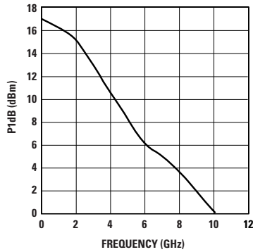
Figure 2. P1dB vs. Frequency at I_d = 50 mA.
