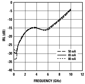
Figure 14. Input Return Loss vs. I_d and Frequency.
