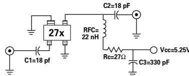
Figure 5. Schematic of 1.9 GHz Circuit.
