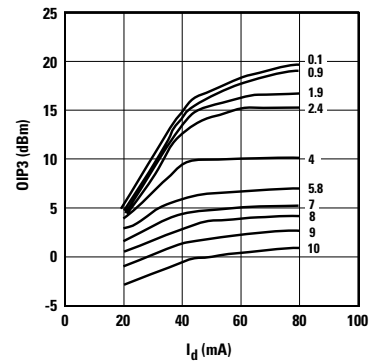
Figure 12. P1dB vs. I_d and Frequency (GHz).
