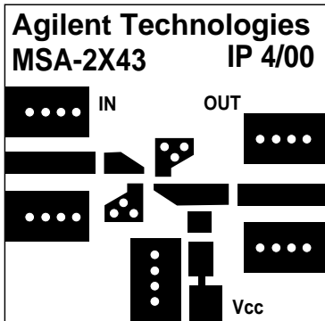
Figure 3. Multi-purpose Evaluation Board.
