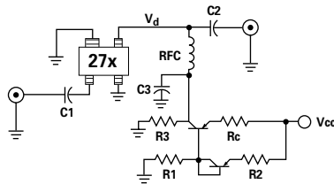
Figure 4. Active Bias Circuit.
