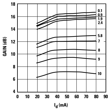
Figure 10. Gain vs. I_d and Frequency (GHz).
