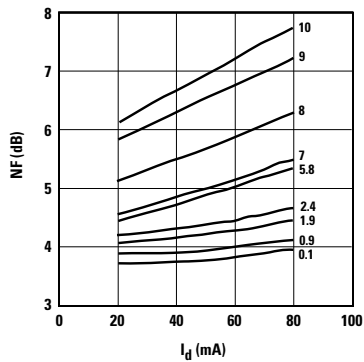
Figure 11. NF vs. I_d and Frequency (GHz).
