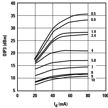
Figure 13. OIP3 vs. I_d and Frequency (GHz).
