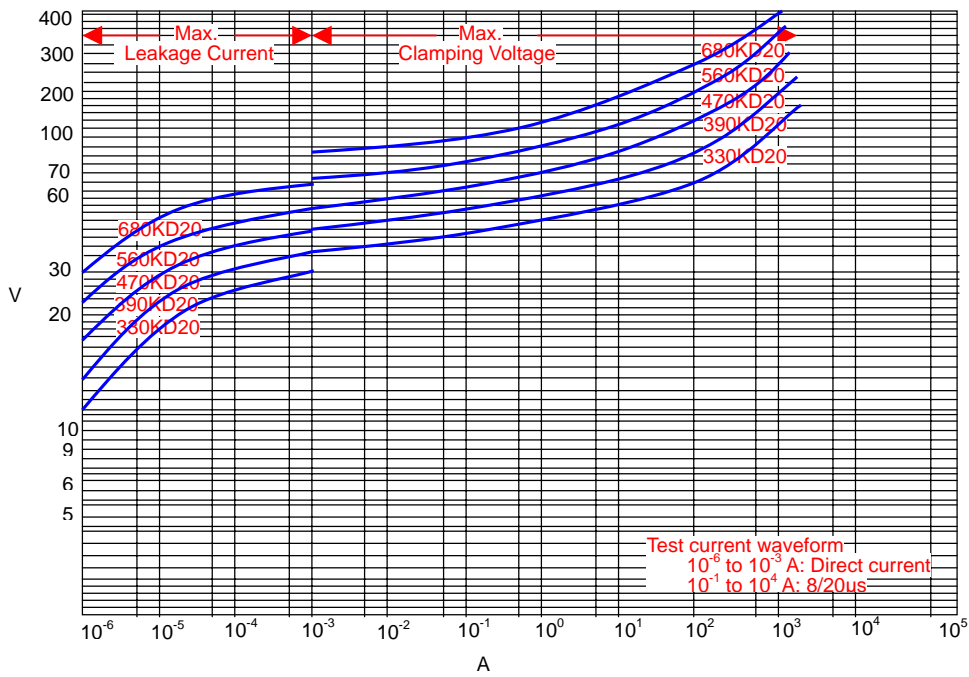
V-I Curve (330K to 680K)
