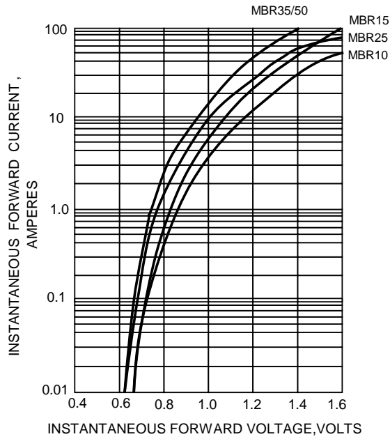
FIG.4-TYPICAL FORWARD CHARACTERISTICS
