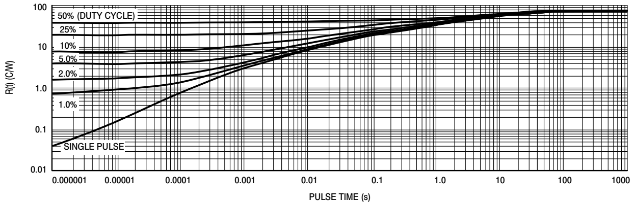
Figure 9. Thermal Response, Junction-to-Ambient (1 in² pad)
