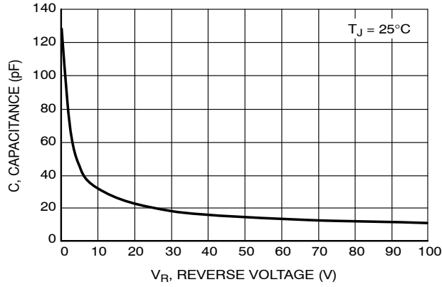
Figure 7. Capacitance
