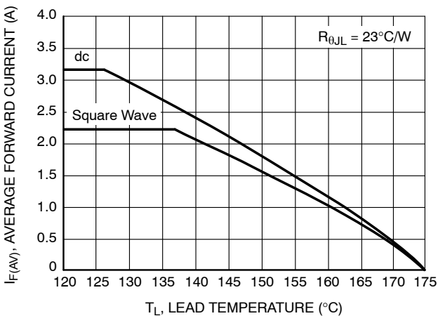
Figure 5. Current Derating
