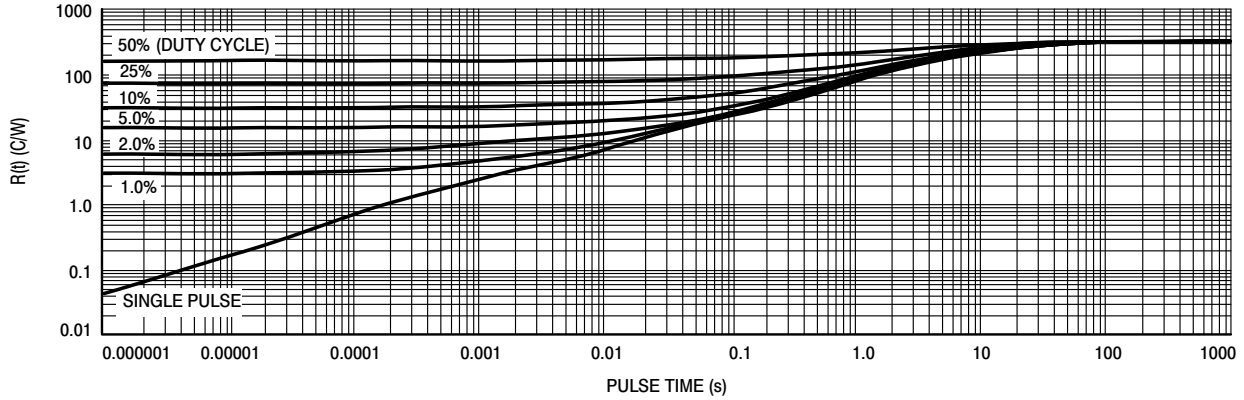
Figure 8. Thermal Response, Junction-to-Ambient (20 mm² pad)
