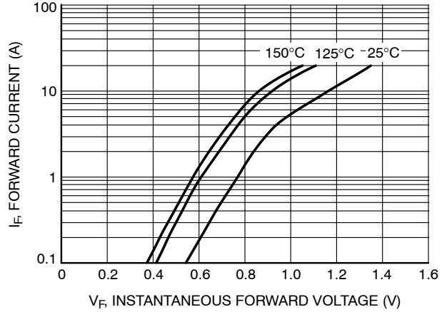
Figure 2. Maximum Forward Voltage
