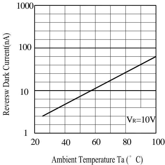
Fig.3 Dark Current vs. Ambient Temperature
