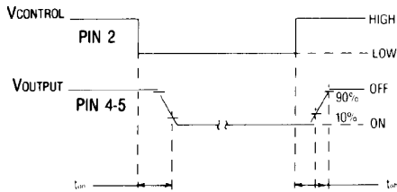
OUTPUT TURN-ON AND TURN-OFF TIMING FIGURE 5
