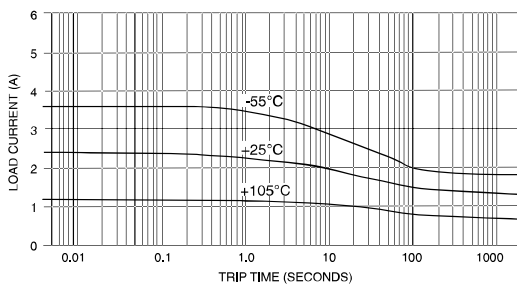
TRIP CURRENT VS TIME FIGURE 7 (SEE NOTE 6)
