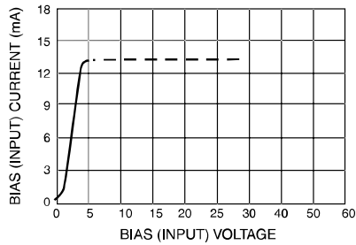
INPUT CURRENT VS VOLTAGE FIGURE 2 (SEE NOTE 4)
