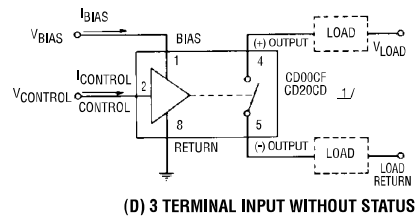
WIRING CONFIGURATIONS FIGURE 1 (SEE NOTE 8)
