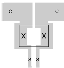
Fig. 1A: Recommended Kelvin layout.
