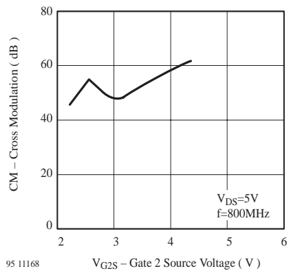
Figure 8. Cross Modulation vs. Gate 2 Source Voltage
