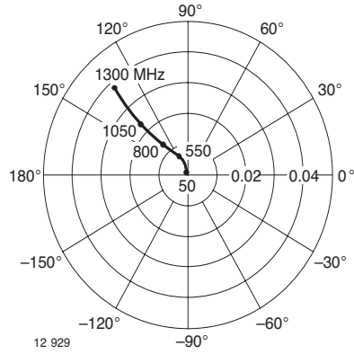
Figure 11. Reverse Transmission Coefficient
