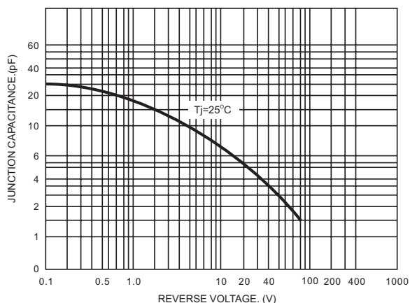
FIG.2- JUNCTION CAPACITANCE
