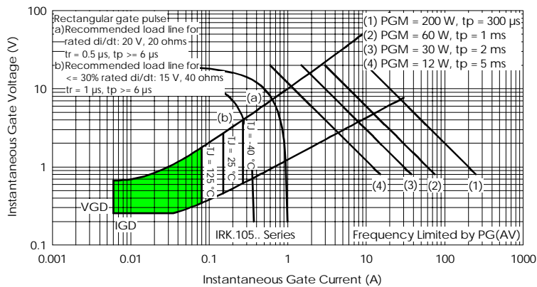
Fig. 13- Gate Characteristics
