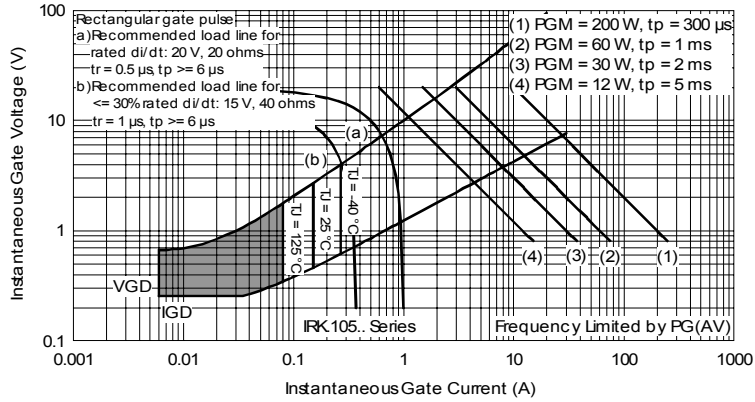
Fig. 14- Gate Characteristics
