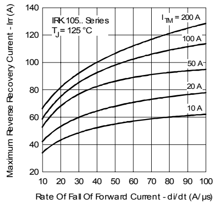
Fig. 12 - Recovery Current Characteristics
