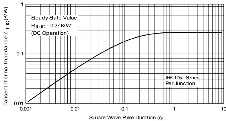
Fig. 13 - Thermal Impedance Z_{thJC} Characteristics
