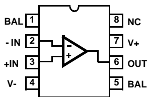
HFA-0002 (PDIP, CDIP, SOIC) TOP VIEW
