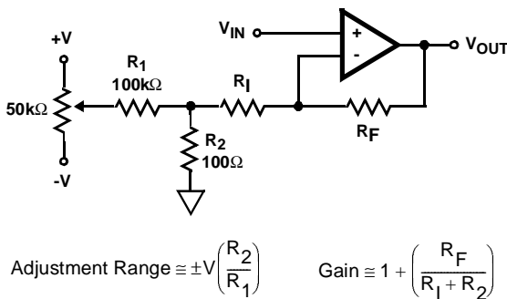
FIGURE 29. NON-INVERTING GAIN
