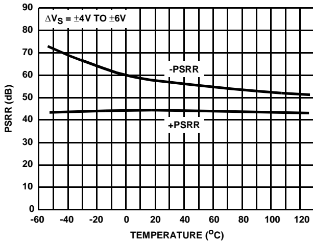
FIGURE 18. PSRR vs TEMPERATURE
