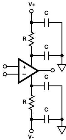
FIGURE 33. IMPROVED DECOUPLING/CURRENT LIMITING
