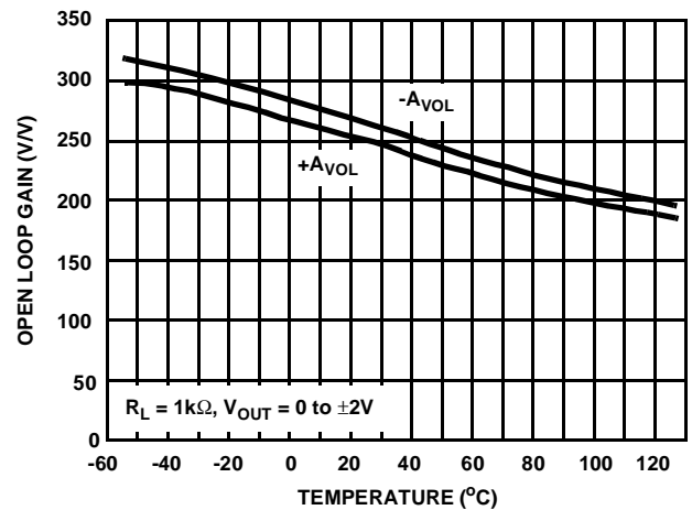
FIGURE 13. OPEN LOOP GAIN vs TEMPERATURE
