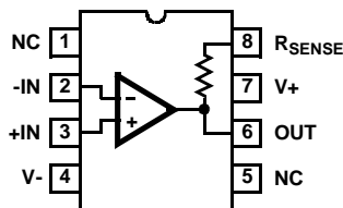
HFA-0005 (PDIP, CDIP, SOIC) TOP VIEW
