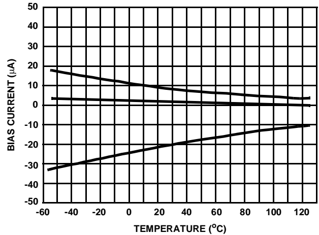
FIGURE 11. BIAS CURRENT vs TEMPERATURE (3 REPRESENTATIVE UNITS)
