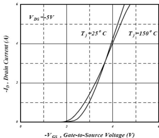
Fig 11. Transfer Characteristics
