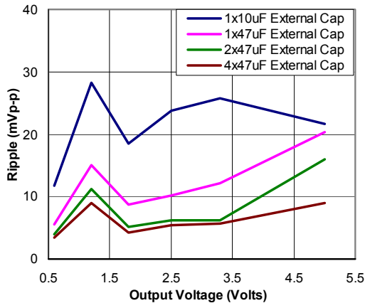
Figure 41. Output ripple voltage for various output voltages with external 1x10 \mu\text{F} , 1x47 \mu\text{F} , 2x47 \mu\text{F} or 4x47 \mu\text{F} ceramic capacitors at the output (20A load). Input voltage is 12V.
