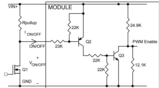
Figure 42. Circuit configuration for using positive On/Off logic.
