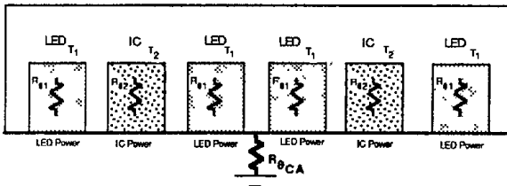
FIGURE 5. THERMAL MODEL
