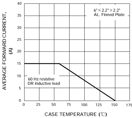
FIG. 1 - MAXIMUM OUTPUT RECTIFIED CURRENT
