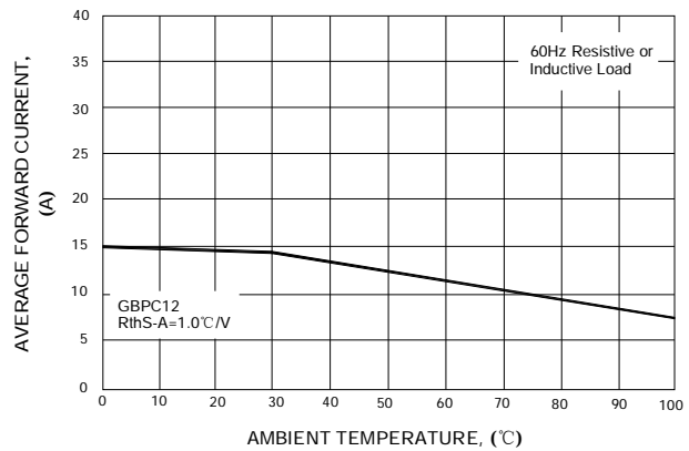
FIG. 2 - MAXIMUM OUTPUT RECTIFIED CURRENT
