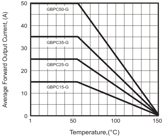
Fig.1 - De-rating Current Output Rectified Current
