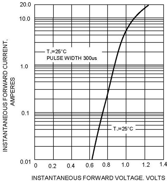
FIG.3-TYPICAL FORWARD CHARACTERISTICS
