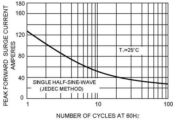
FIG.1-MAXIMUM NON-REPETITIVE SURGE CURRENT
