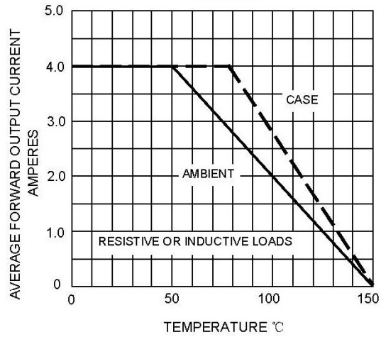
FIG.2-FORWARD DERATING CURRENT
