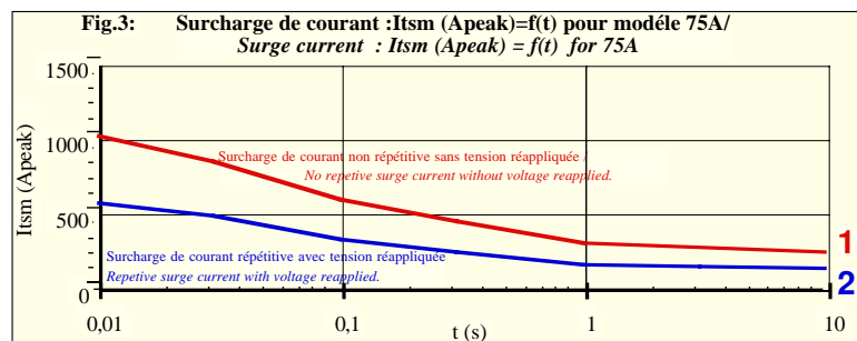
fig 3 : Courants de surcharges / Overload currents
