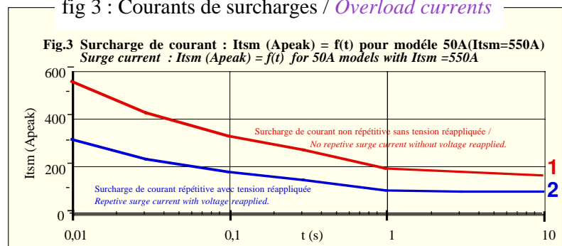
fig 3 : Courants de surcharges / Overload currents
