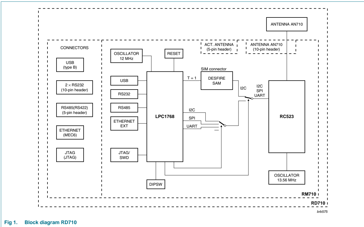
Fig 1. Block diagram RD710
