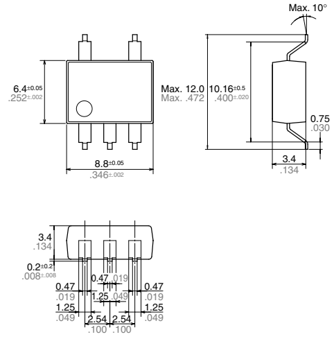
Surface mount terminal type
