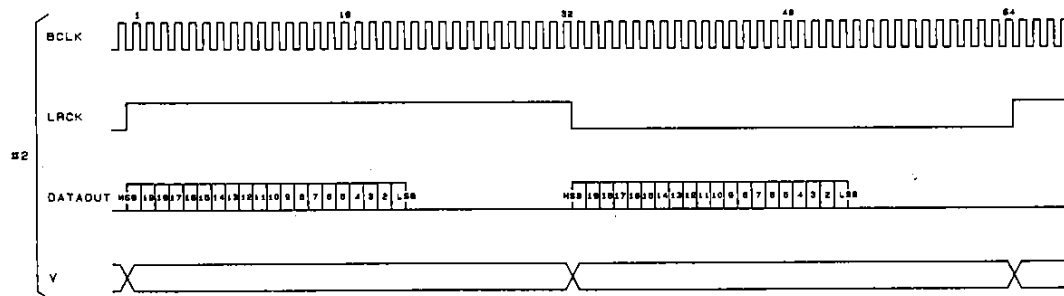
Timing chart #1 is for 16-bit MSB first output mode. Timing chart #2 is for 20-bit MSB first output mode.
