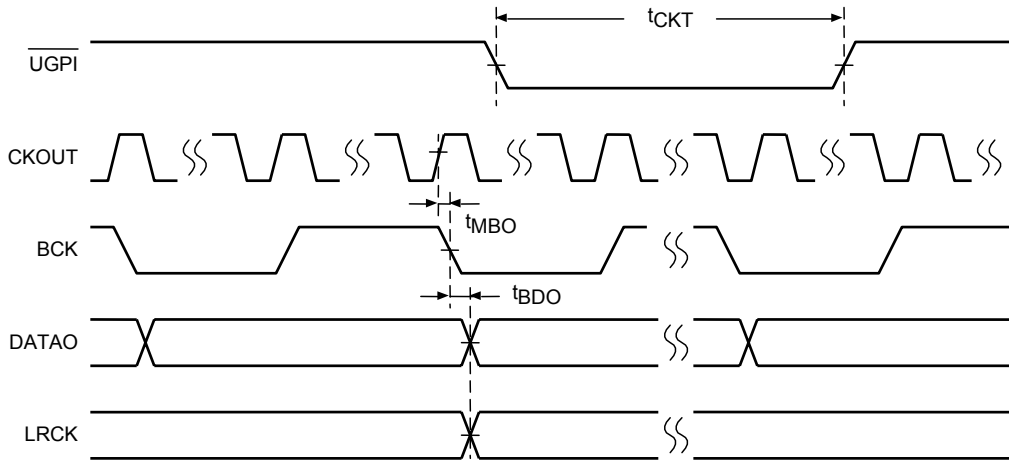
Figure 7.1 AC Characteristics
