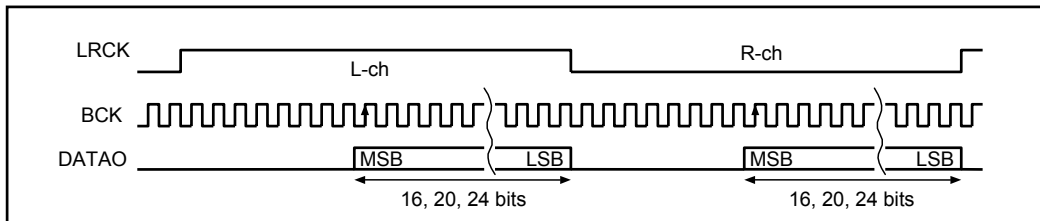
(2) : MSB first right-justified data output (OFSEL[2 : 0]=010, 011 or 100)
