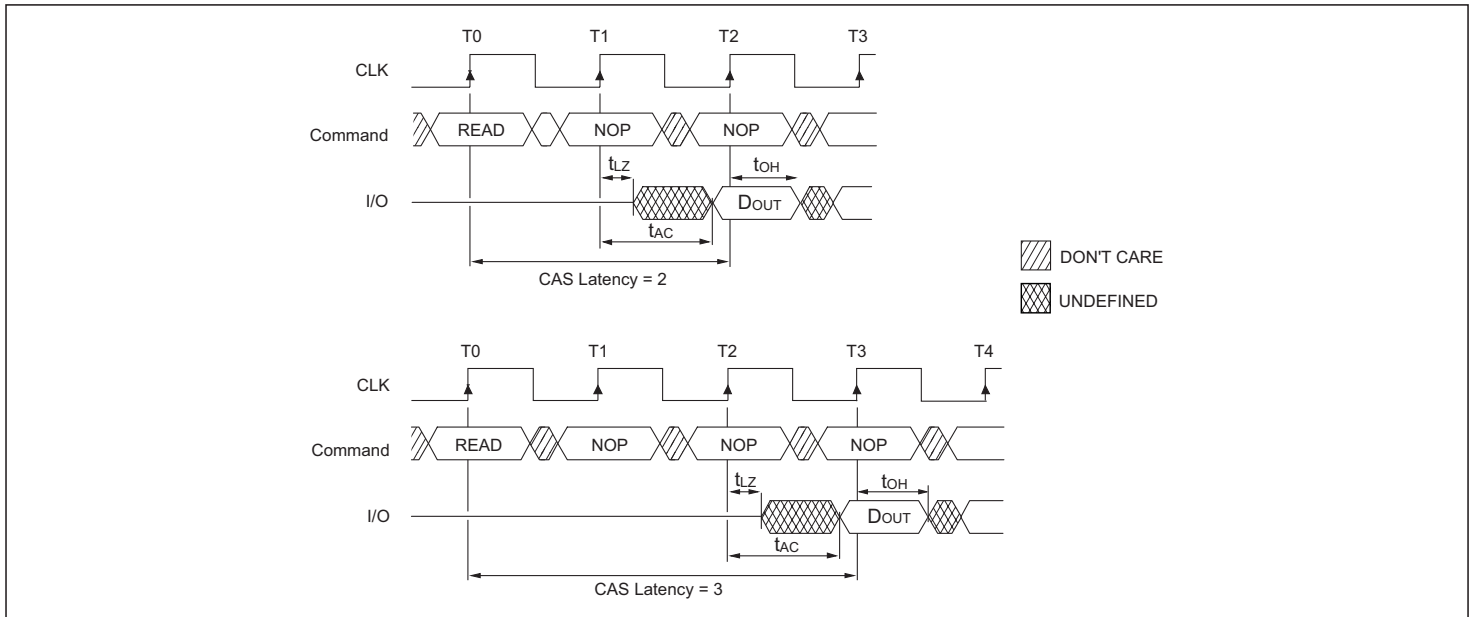
FIGURE 4 – CAS LATENCY
