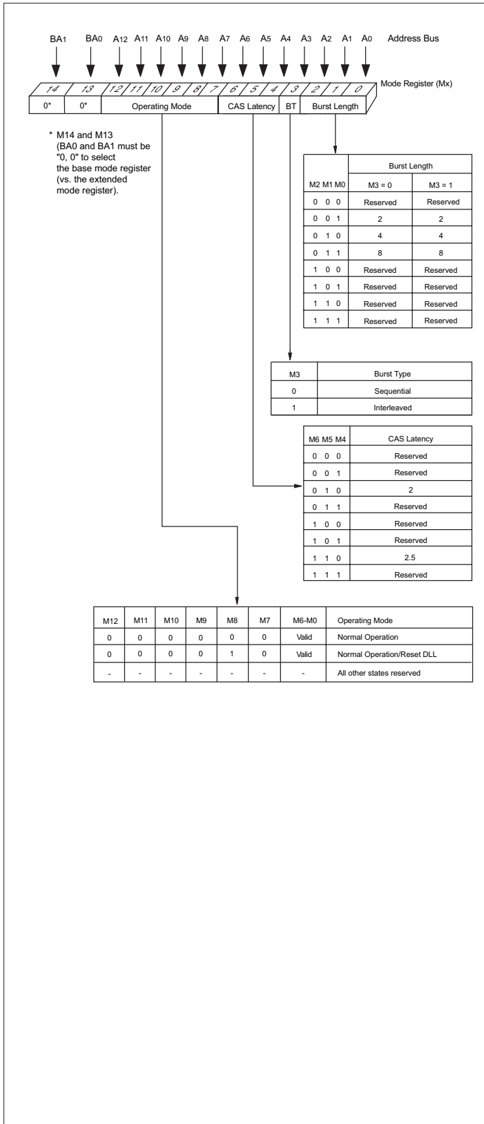
FIGURE 3 – MODE REGISTER DEFINITION
