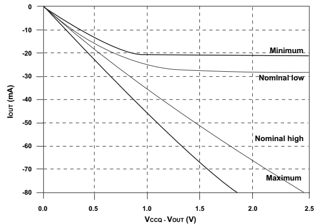
FIGURE D – PULL-UP CHARACTERISTICS
