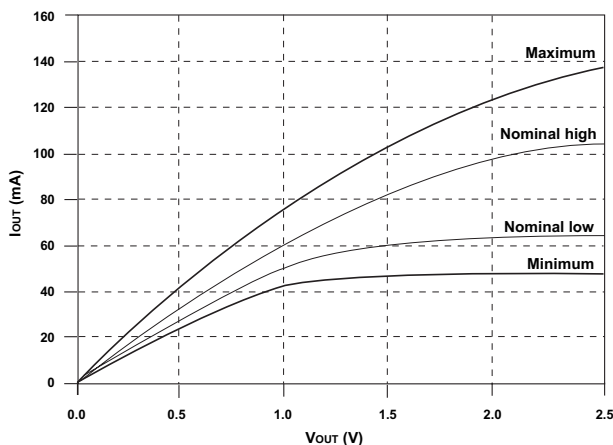
FIGURE A – PULL-DOWN CHARACTERISTICS
