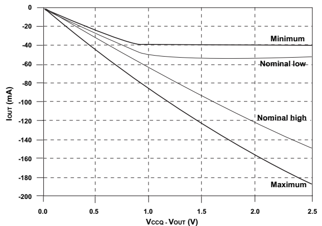
FIGURE B – PULL-UP CHARACTERISTICS
