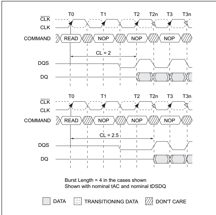
FIGURE 4 – CAS LATENCY
