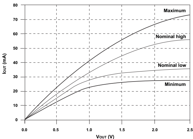
FIGURE C – PULL-DOWN CHARACTERISTICS
