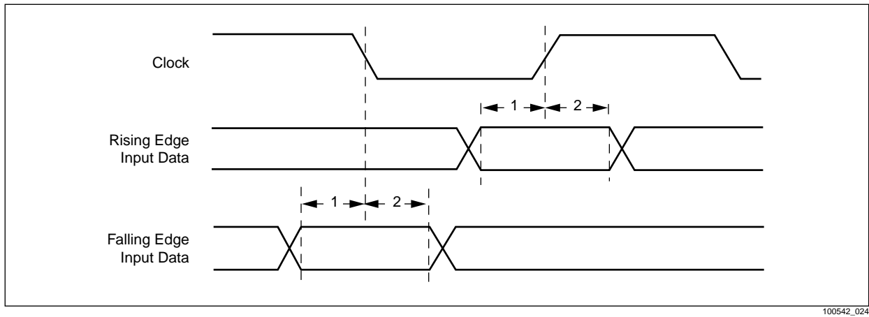
Figure 4-3. Line Side Receiver Input Data Setup/Hold Timing (1 = tsu [setup time]; 2 = thld [hold time])
