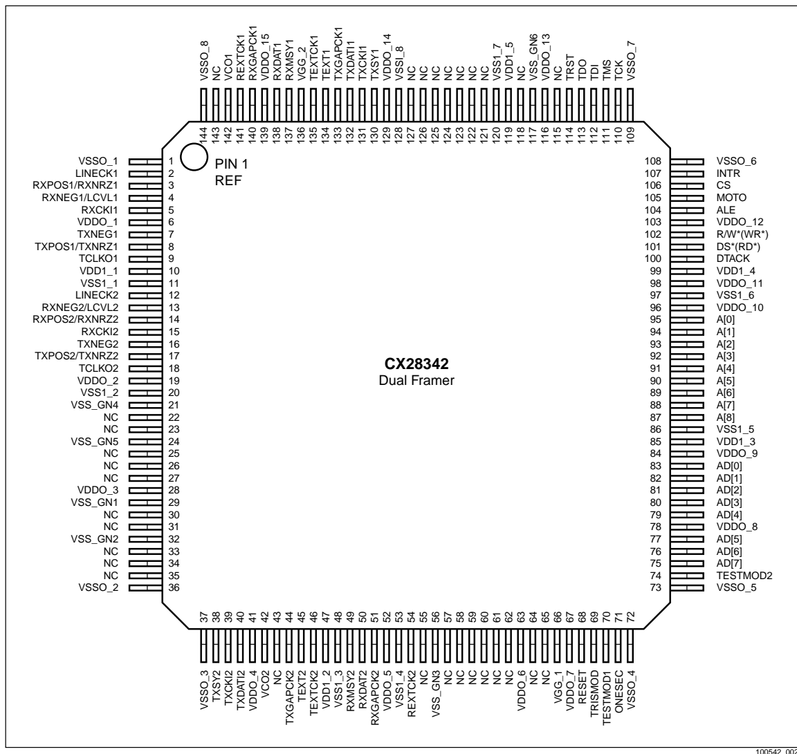
Figure 1-1. CX28342 Pin Assignments
