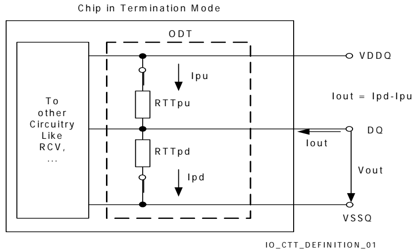
On-Die Termination : Definition of Voltages and Currents
