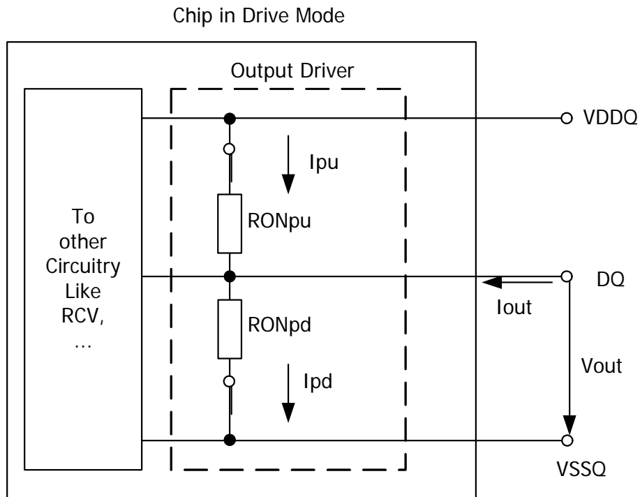
Output Driver: Definition of Voltages and Currents
