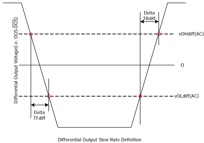
Fig. Differential Output Slew Rate Definition
